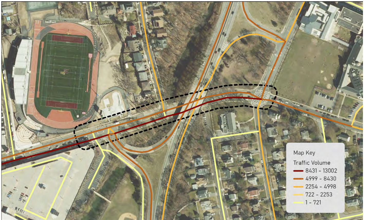
Figure 3: Traffic volume during a Fall weekday in 2023. Source: ReplicaHQ
