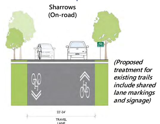
Conceptual Cross Section
