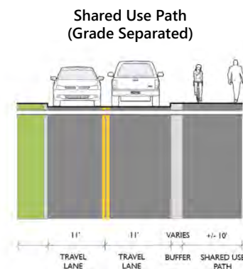
Conceptual Cross Section
