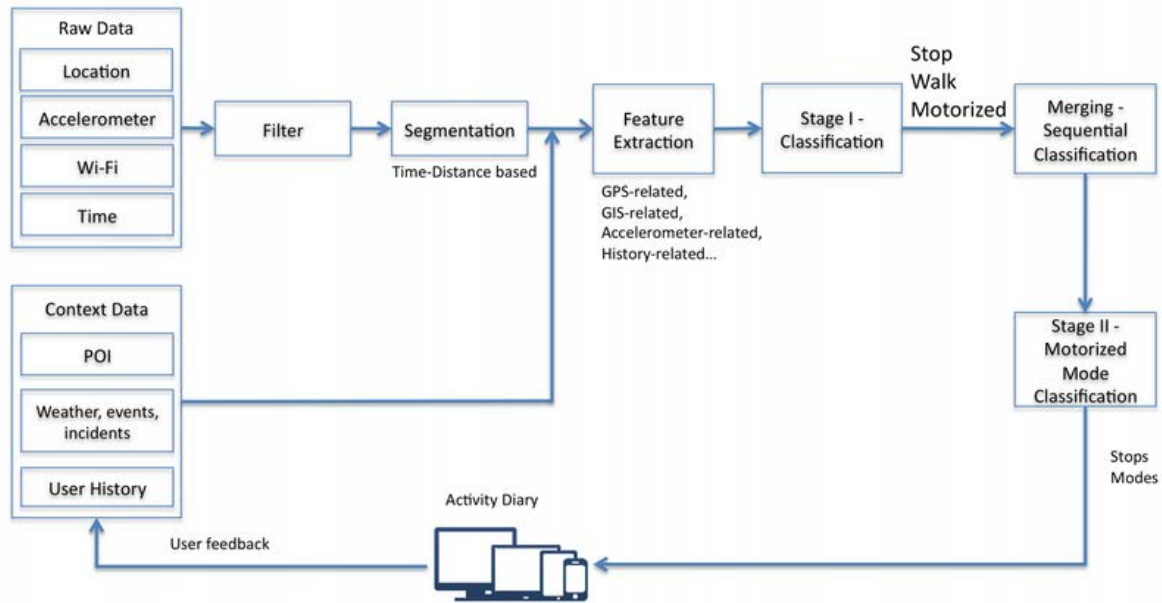
Figure 5 -- System Architecture
